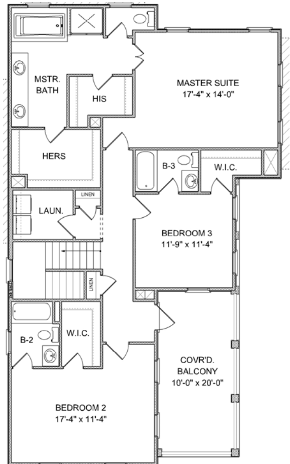
UPPER LEVEL
